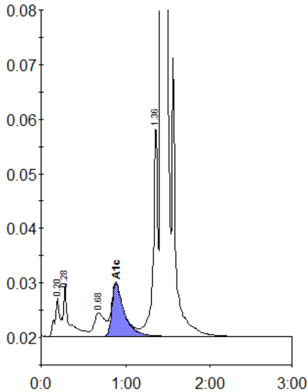
Peak table - ID: 10413319
